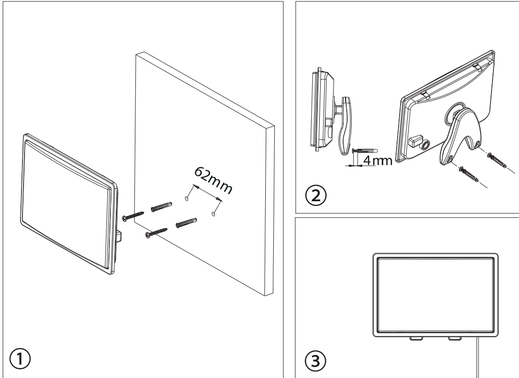
Wall-mounted installation
