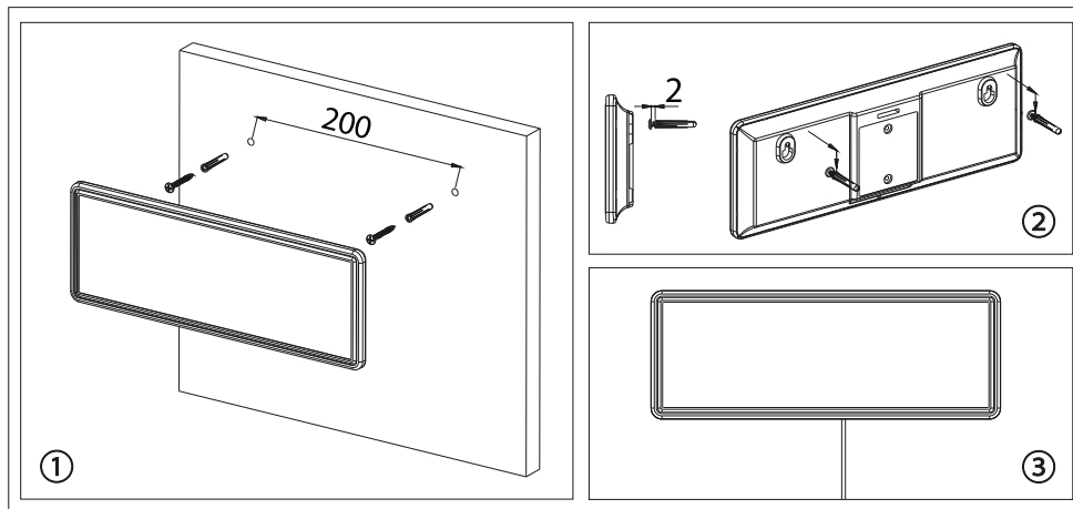
Wall-mounted installation
